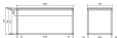
Office Table 160 x 70 x 77 cm
